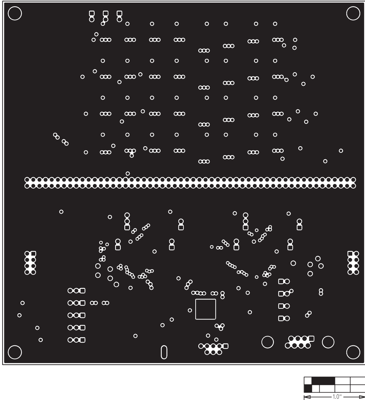
Figure 8. MAX6974 EV Kit PCB Layout—Ground Layer 2
