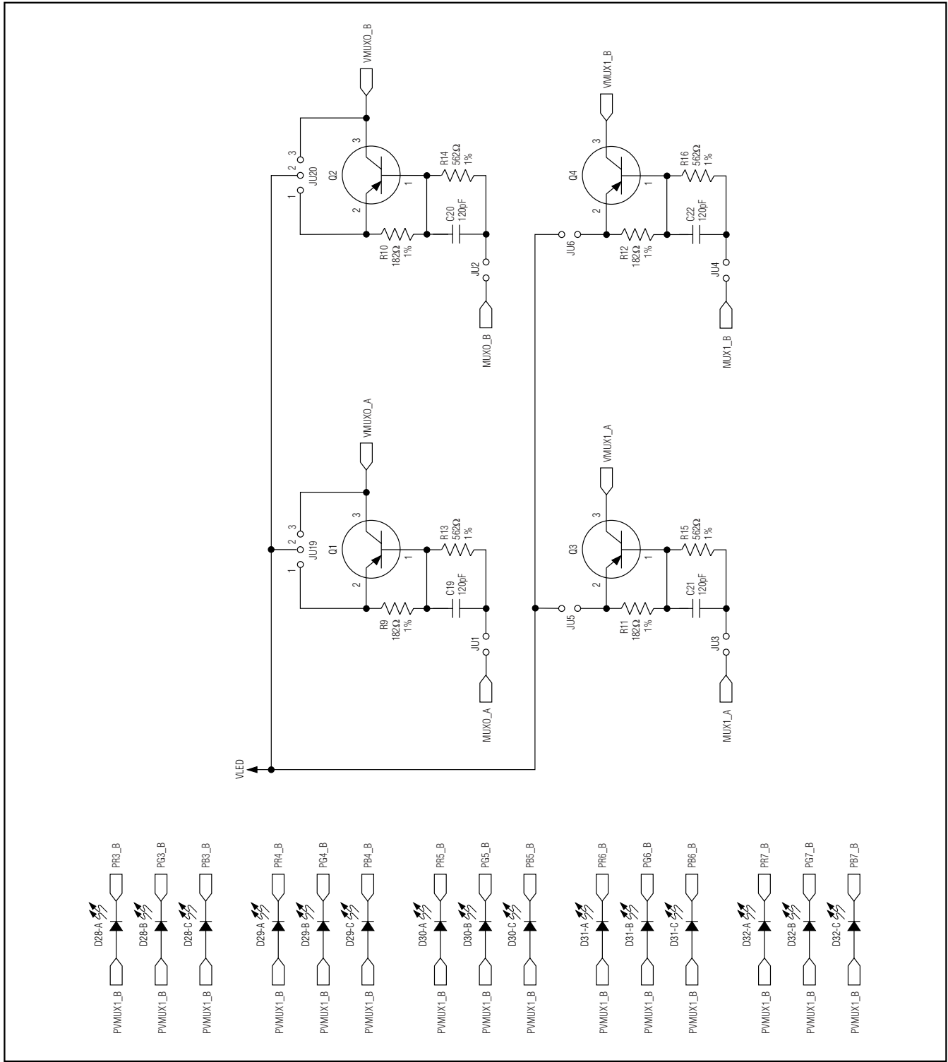
Figure 5d. MAX6974 EV Kit Schematic (Sheet 4 of 5)
